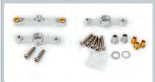
TT-01 Alu Lenkung komplett TT-01 Alum. Steering Assembly Set
